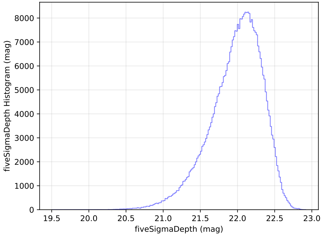
internal_u_expt38_nscale1.1v3.4_10yrs All sky y band: fiveSigmaDepth Histogram
