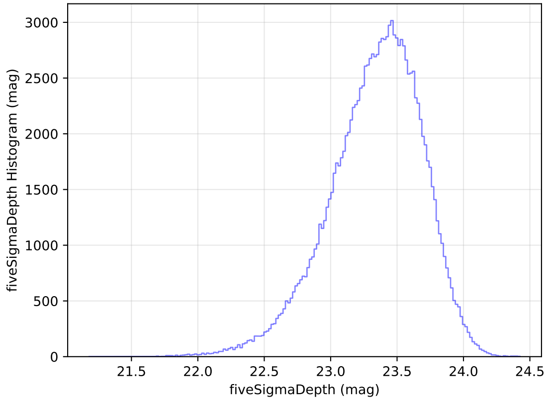
internal_u_expt38_nscale1.1v3.4_10yrs All sky u band: fiveSigmaDepth Histogram
