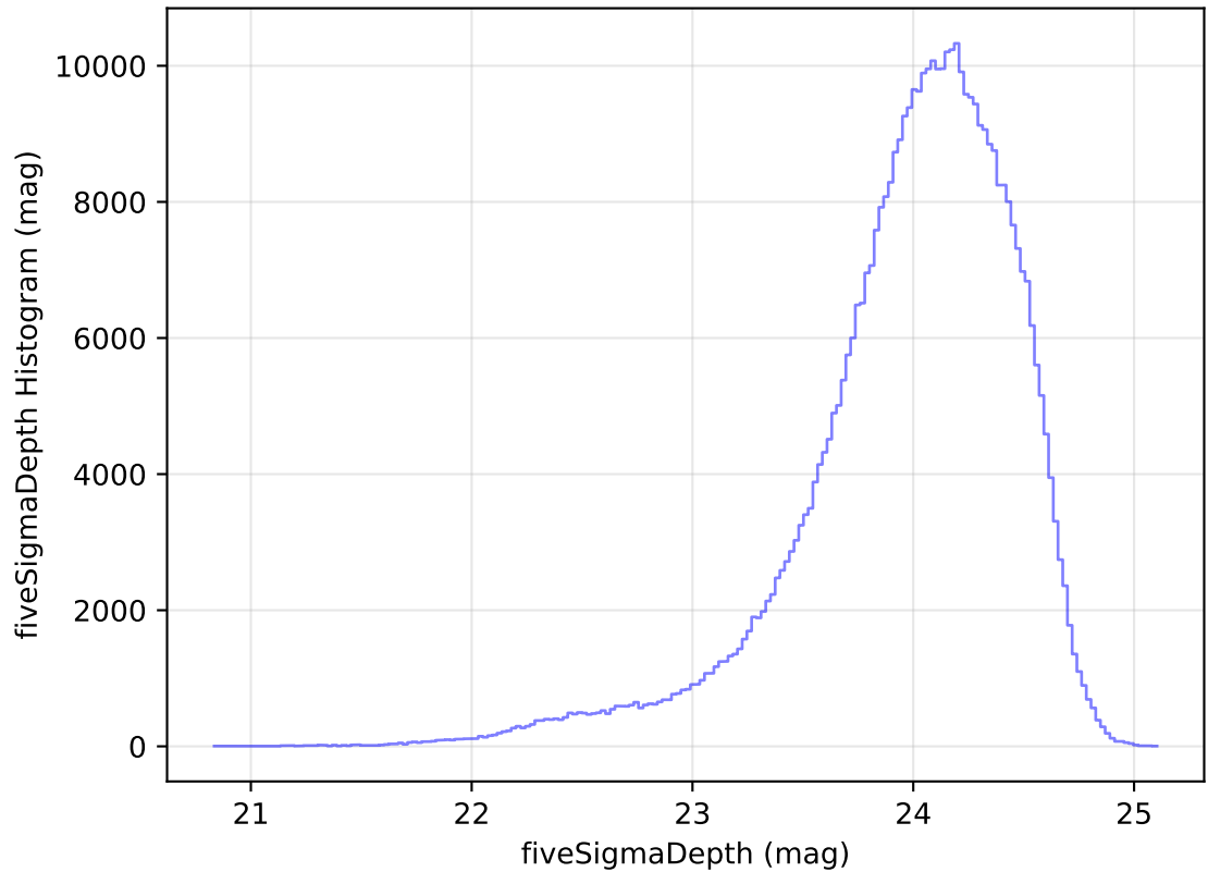
internal_u_expt38_nscale1.1v3.4_10yrs All sky r band: fiveSigmaDepth Histogram
