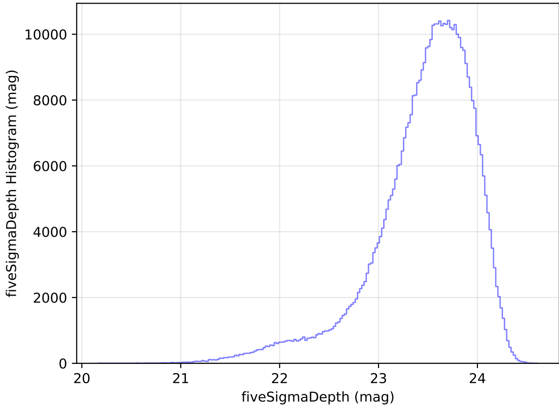
internal_u_expt38_nscale1.1v3.4_10yrs All sky i band: fiveSigmaDepth Histogram
