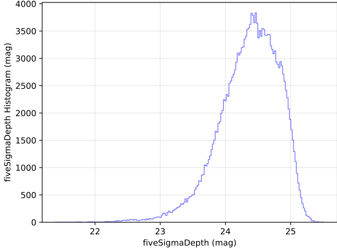
internal_u_expt38_nscale1.1v3.4_10yrs All sky g band: fiveSigmaDepth Histogram
