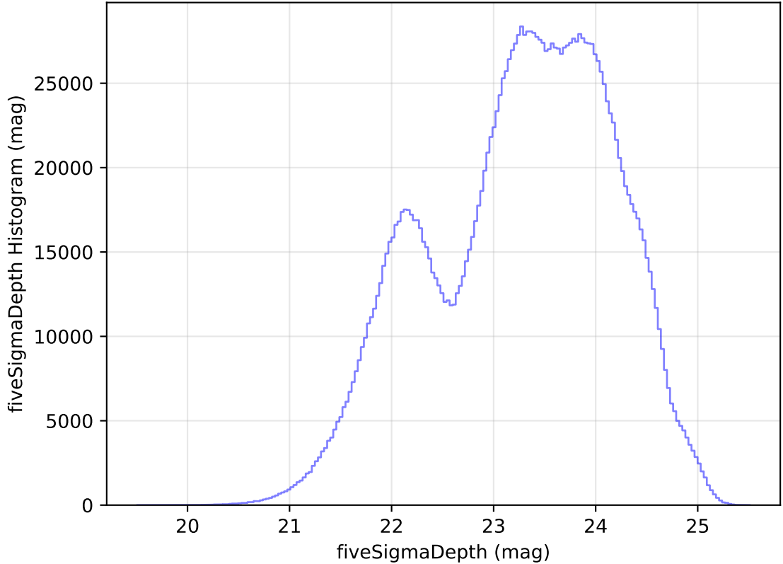
internal_u_expt38_nscale1.1v3.4_10yrs All sky all bands: fiveSigmaDepth Histogram
