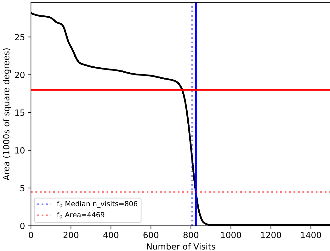
internal_u_expt38_nscale1.1v3.4_10yrs All sky: f0
