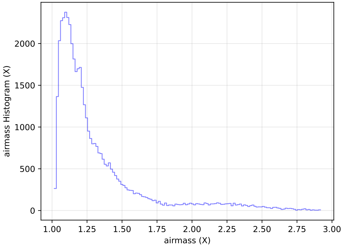
internal_u_expt38_nscale1.1v3.4_10yrs Yr 1 z band: airmass Histogram
