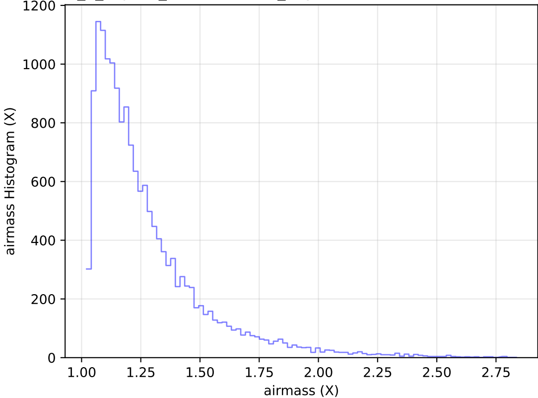
internal_u_expt38_nscale1.1v3.4_10yrs Yr 1 u band: airmass Histogram
