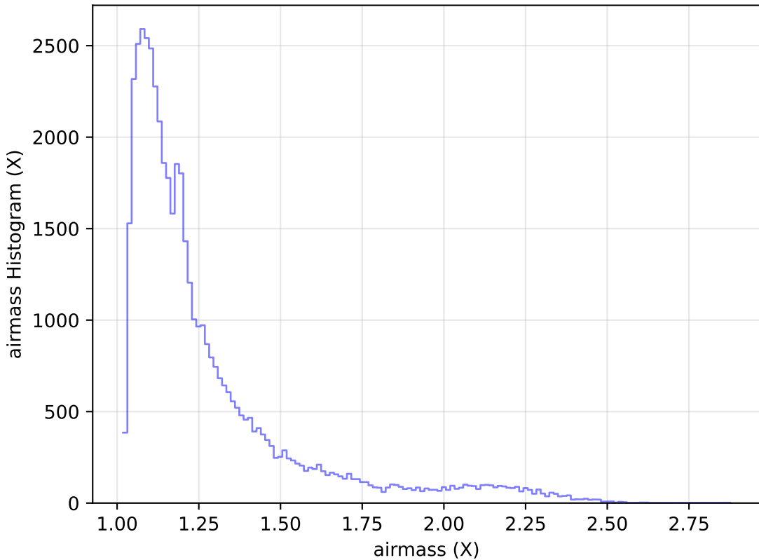
internal_u_expt38_nscale1.1v3.4_10yrs Yr 1 r band: airmass Histogram
