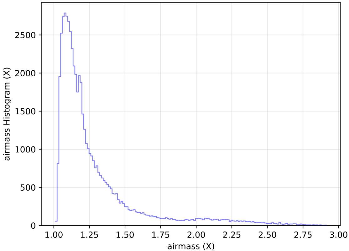
internal_u_expt38_nscale1.1v3.4_10yrs Yr 1 i band: airmass Histogram
