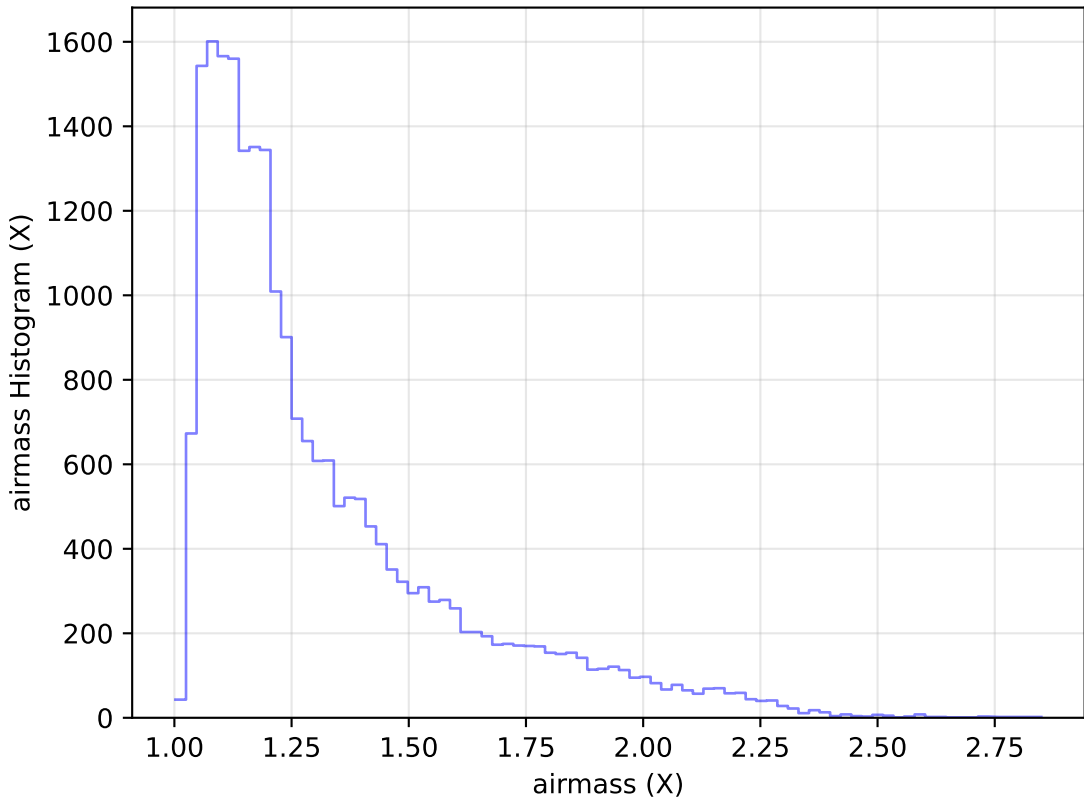
internal_u_expt38_nscale1.1v3.4_10yrs Yr 1 g band: airmass Histogram
