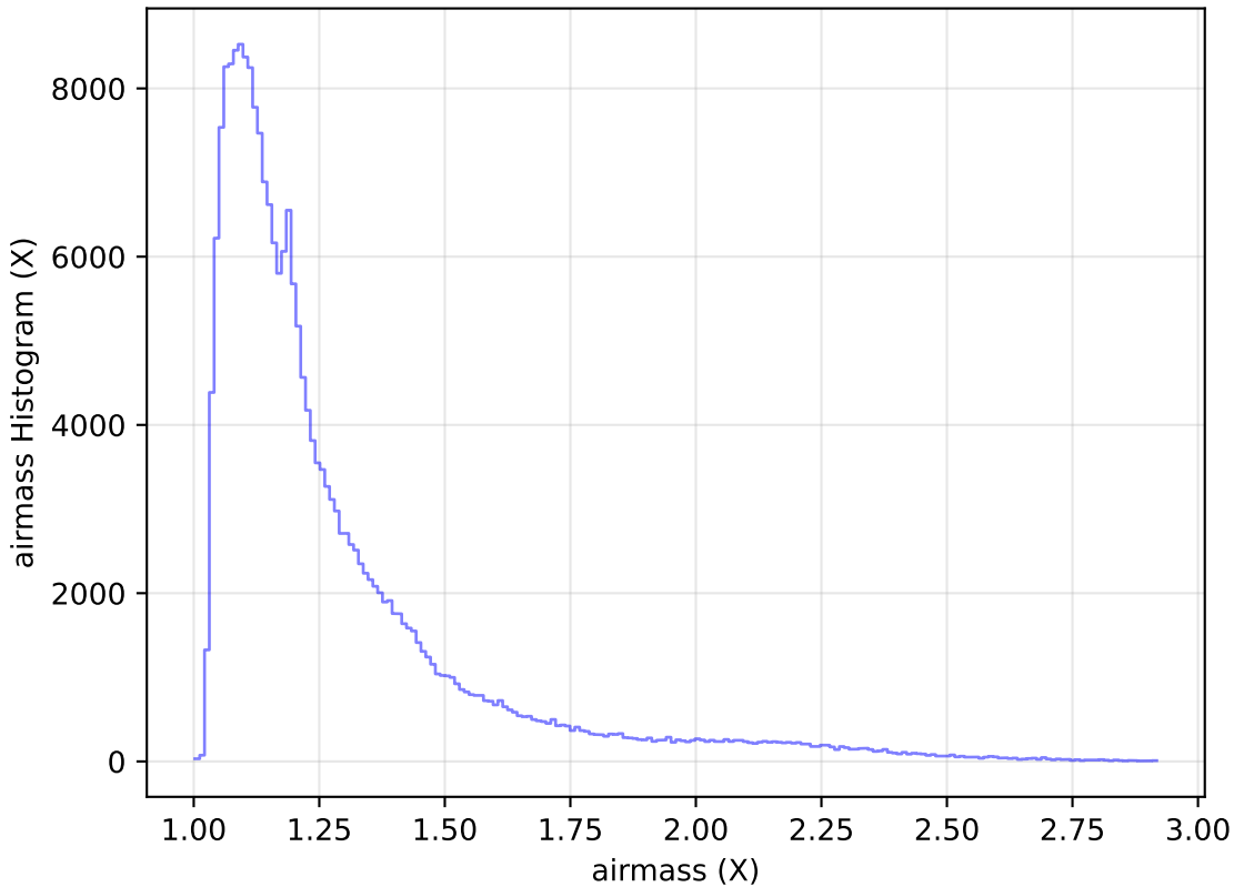
internal_u_expt38_nscale1.1v3.4_10yrs Yr 1 all bands: airmass Histogram
