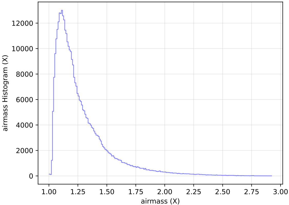
internal_u_expt38_nscale1.1v3.4_10yrs WFD y band: airmass Histogram
