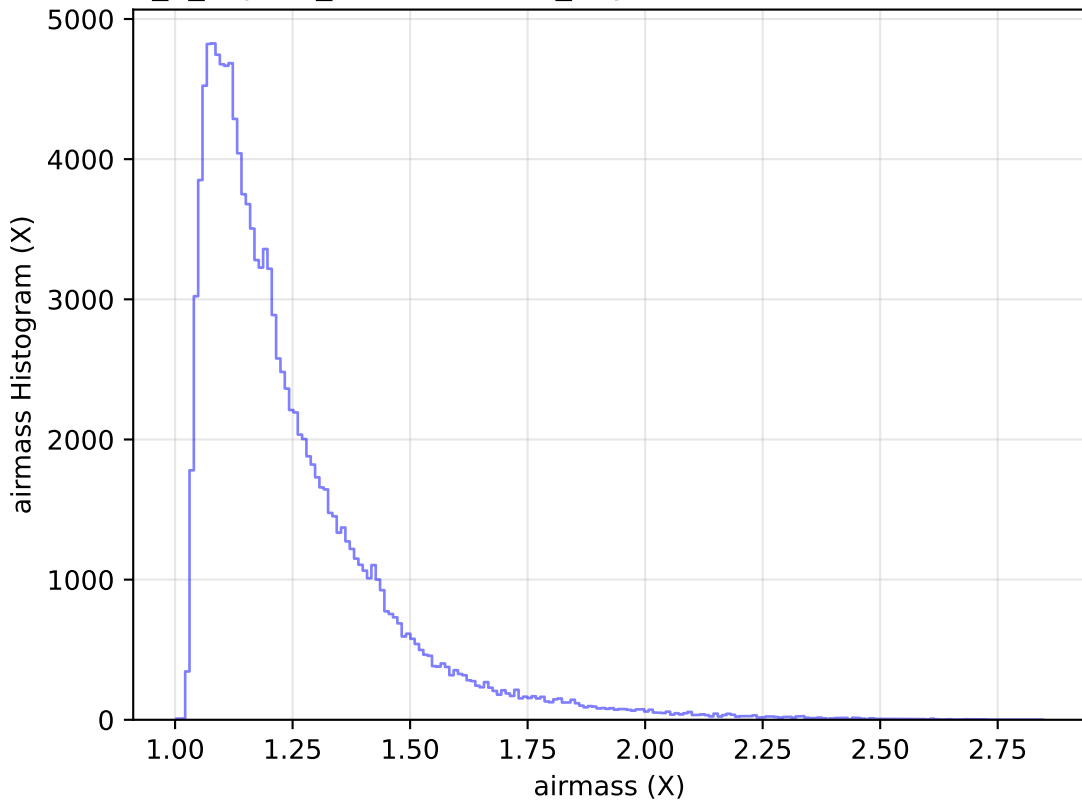
internal_u_expt38_nscale1.1v3.4_10yrs WFD u band: airmass Histogram
