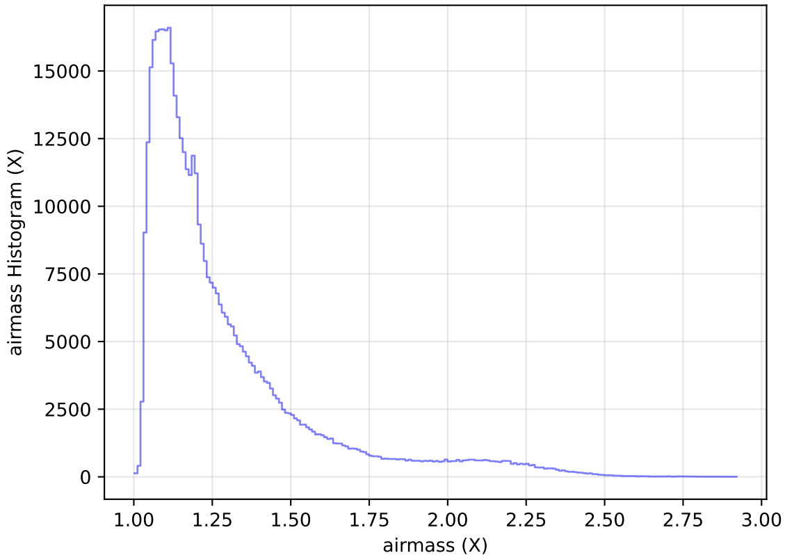
internal_u_expt38_nscale1.1v3.4_10yrs WFD r band: airmass Histogram
