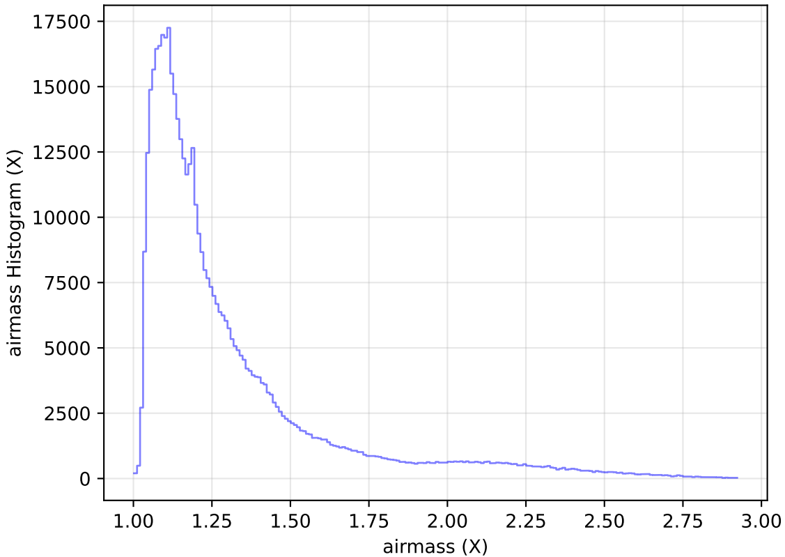
internal_u_expt38_nscale1.1v3.4_10yrs WFD i band: airmass Histogram
