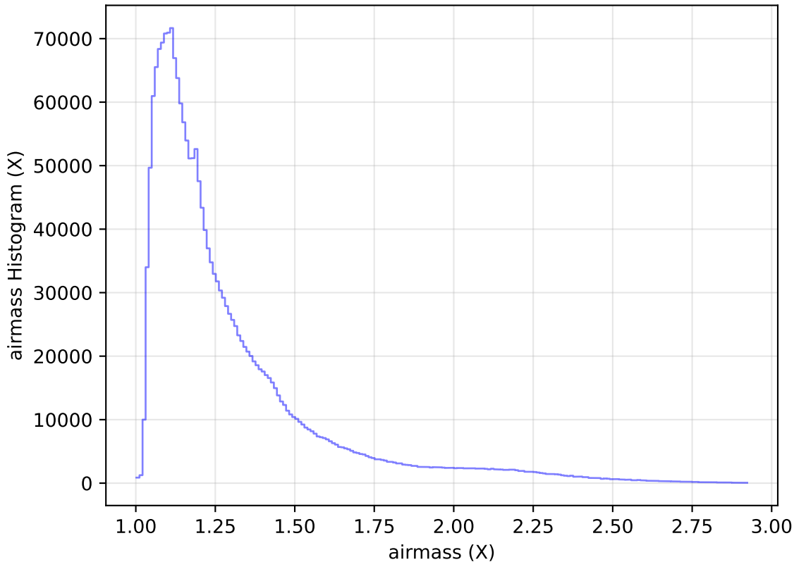
internal_u_expt38_nscale1.1v3.4_10yrs WFD all bands: airmass Histogram
