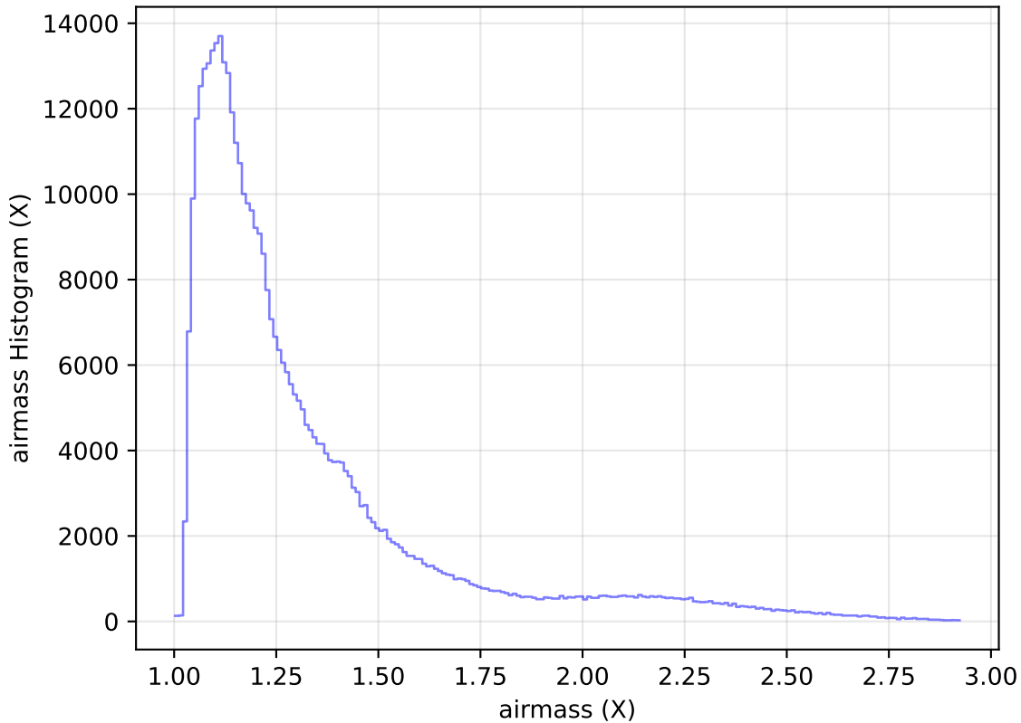
internal_u_expt38_nscale1.1v3.4_10yrs All sky z band: airmass Histogram
