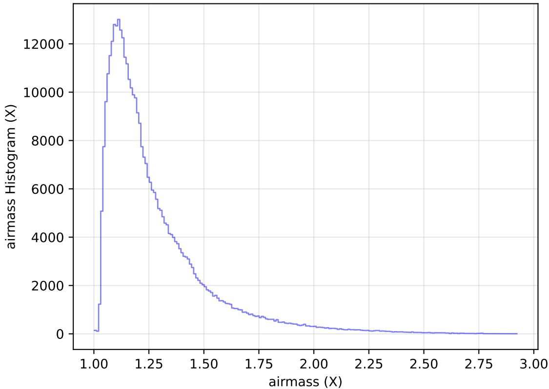
internal_u_expt38_nscale1.1v3.4_10yrs All sky y band: airmass Histogram
