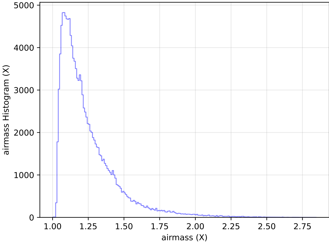
internal_u_expt38_nscale1.1v3.4_10yrs All sky u band: airmass Histogram
