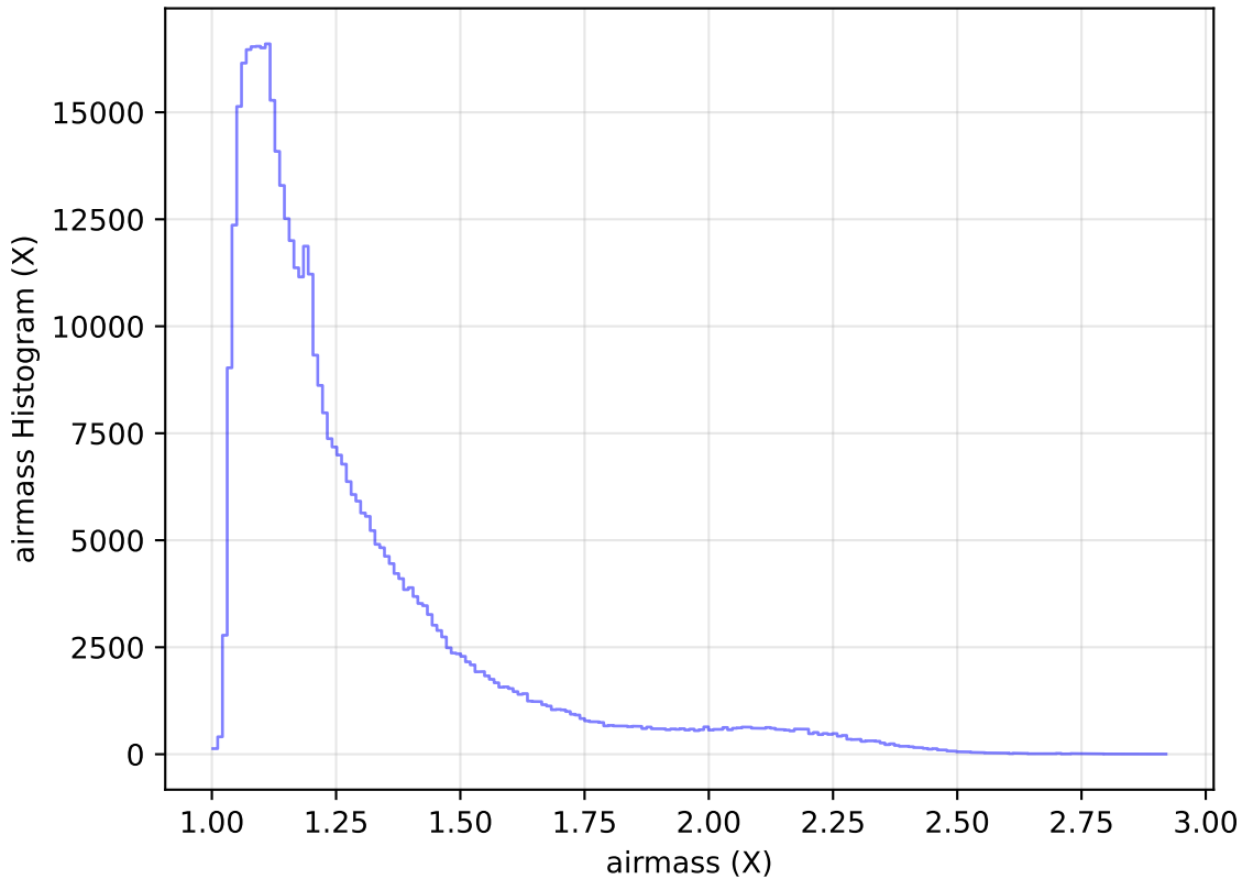
internal_u_expt38_nscale1.1v3.4_10yrs All sky r band: airmass Histogram
