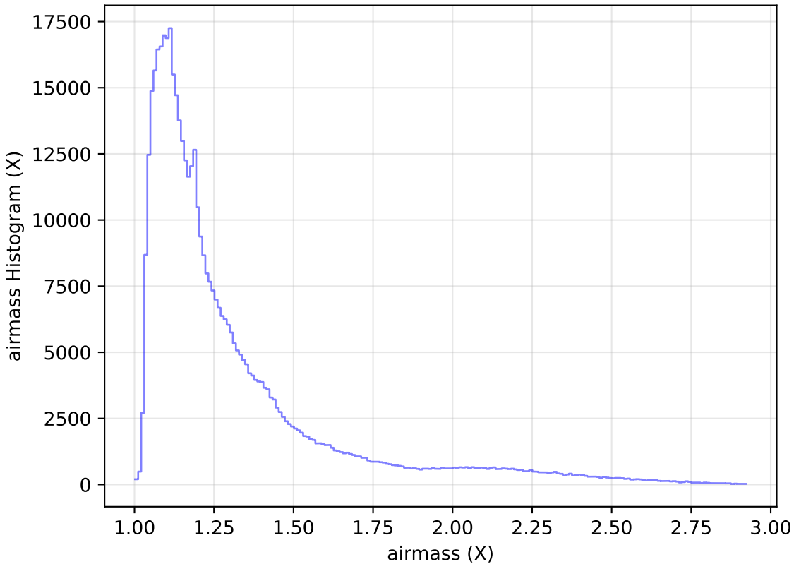
internal_u_expt38_nscale1.1v3.4_10yrs All sky i band: airmass Histogram
