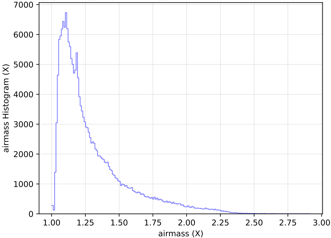
internal_u_expt38_nscale1.1v3.4_10yrs All sky g band: airmass Histogram
