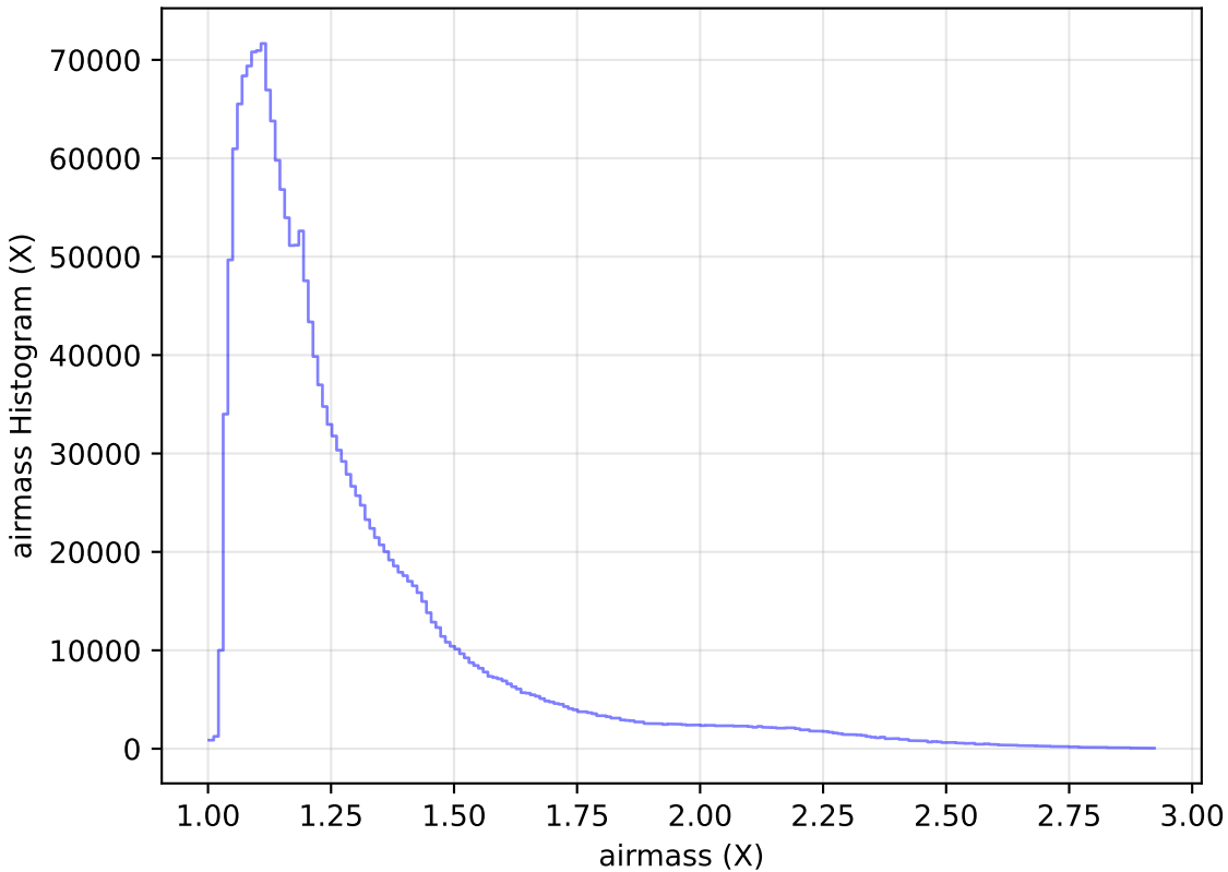
internal_u_expt38_nscale1.1v3.4_10yrs All sky all bands: airmass Histogram
