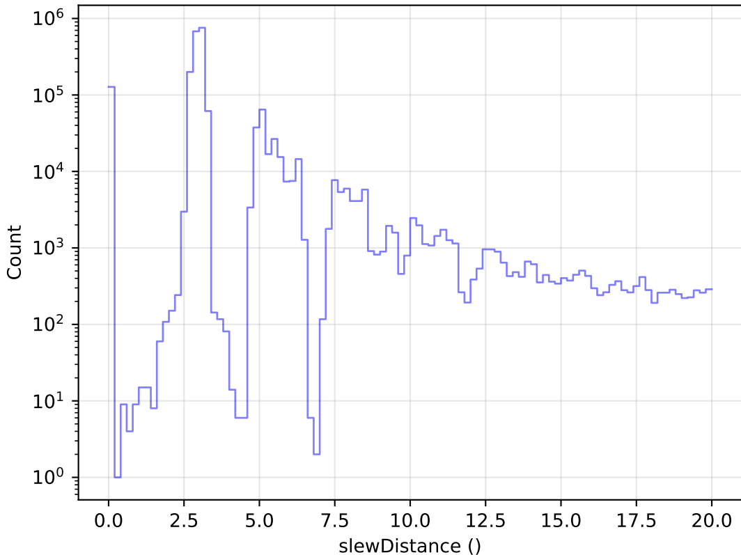
internal_u_expt38_nscale1.1v3.4_10yrs All visits: Zoom Slew Distance Histogram
