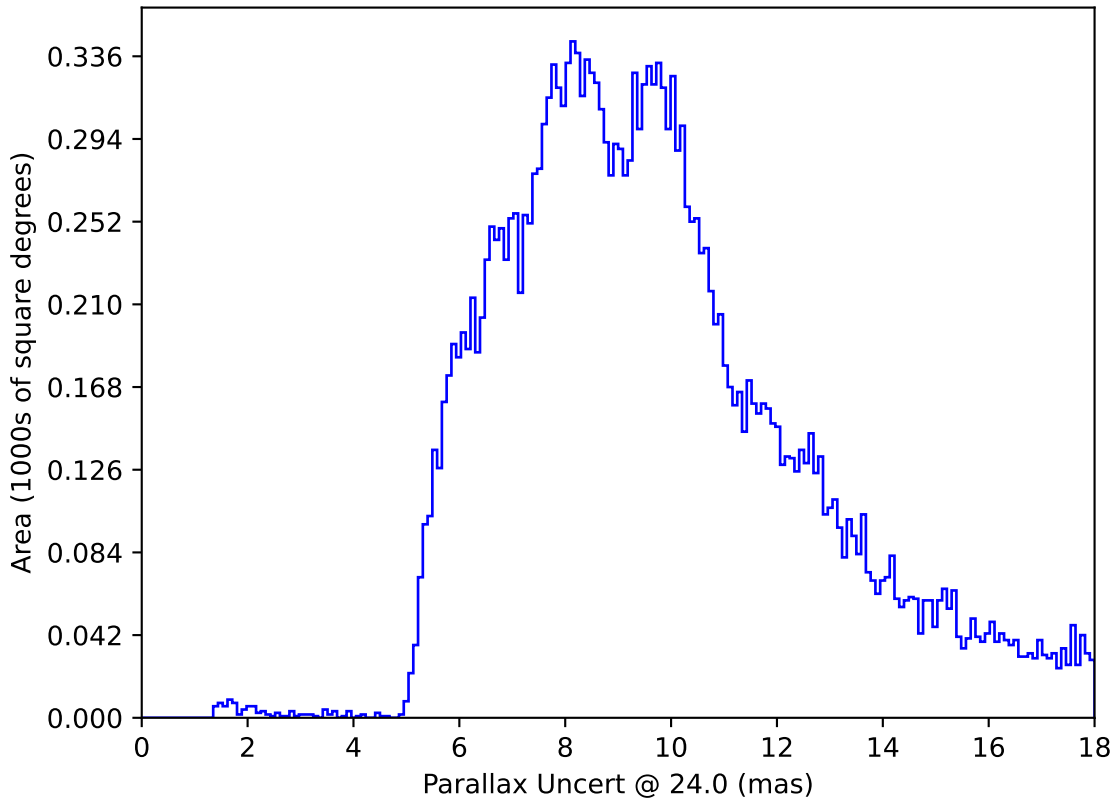
internal_u_expt38_nscale1.1v3.4_10yrs All sky: Parallax Uncert @ 24.0
