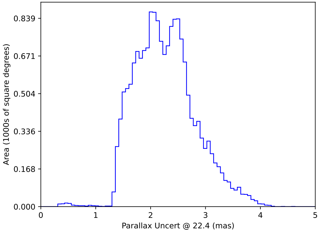
internal_u_expt38_nscale1.1v3.4_10yrs WFD: Parallax Uncert @ 22.4
