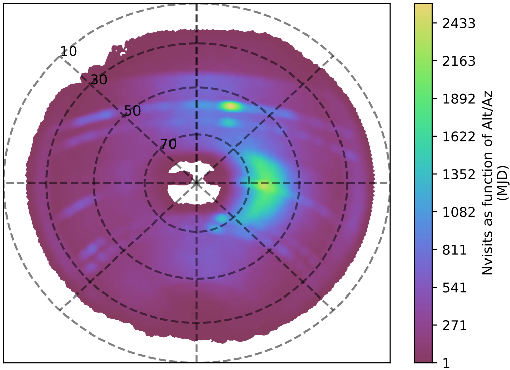
internal_u_expt38_nscale1.1v3.4_10yrs z band: Nvisits as function of Alt/Az
