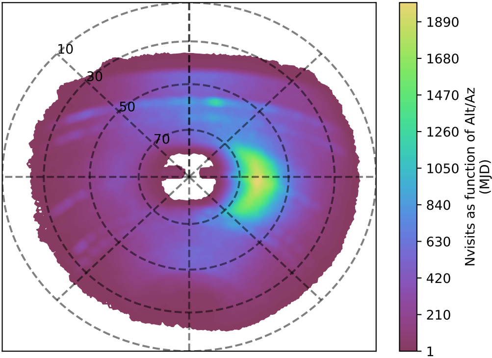
internal_u_expt38_nscale1.1v3.4_10yrs y band: Nvisits as function of Alt/Az
