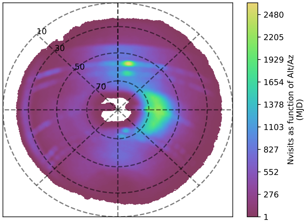
internal_u_expt38_nscale1.1v3.4_10yrs r band: Nvisits as function of Alt/Az
