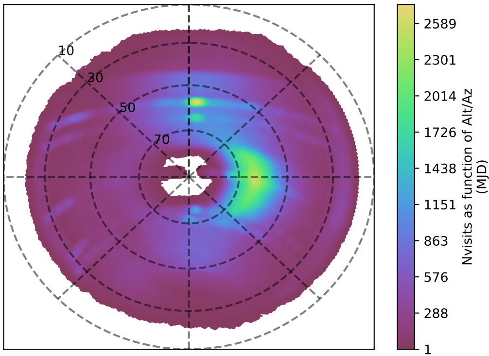
internal_u_expt38_nscale1.1v3.4_10yrs i band: Nvisits as function of Alt/Az
