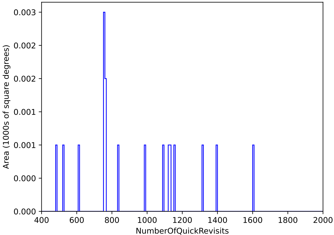
internal_u_expt38_nscale1.1v3.4_10yrs WFD: NumberOfQuickRevisits
