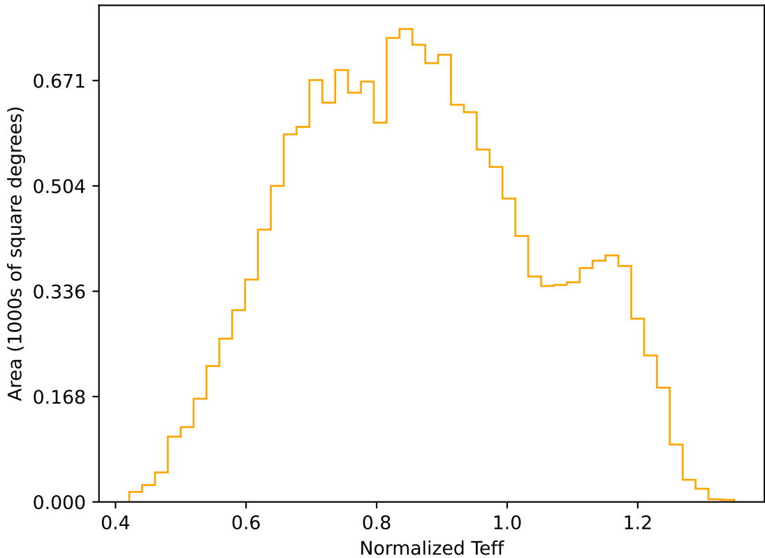
internal_u_expt38_nscale1.1v3.4_10yrs WFD r band: Normalized Teff
