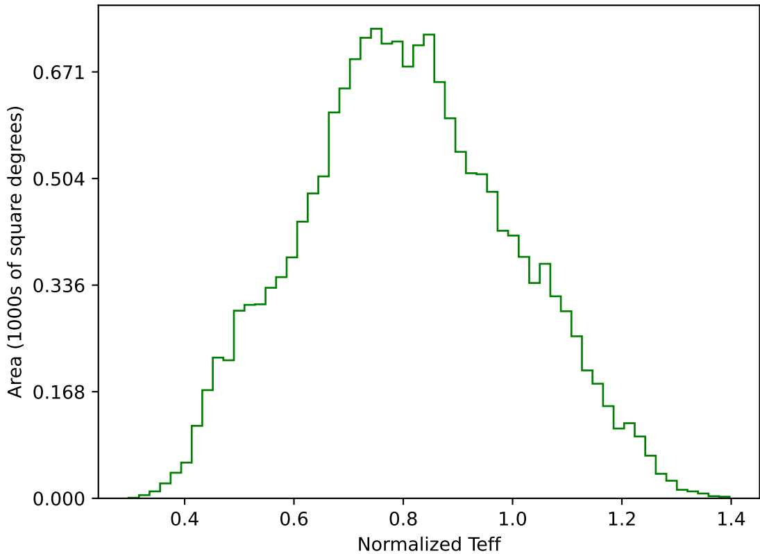
internal_u_expt38_nscale1.1v3.4_10yrs WFD g band: Normalized Teff
