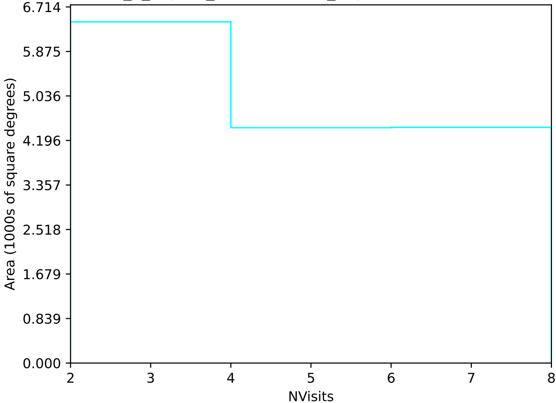
internal_u_expt38_nscale1.1v3.4_10yrs Yr 3-4 u band: NVisits
