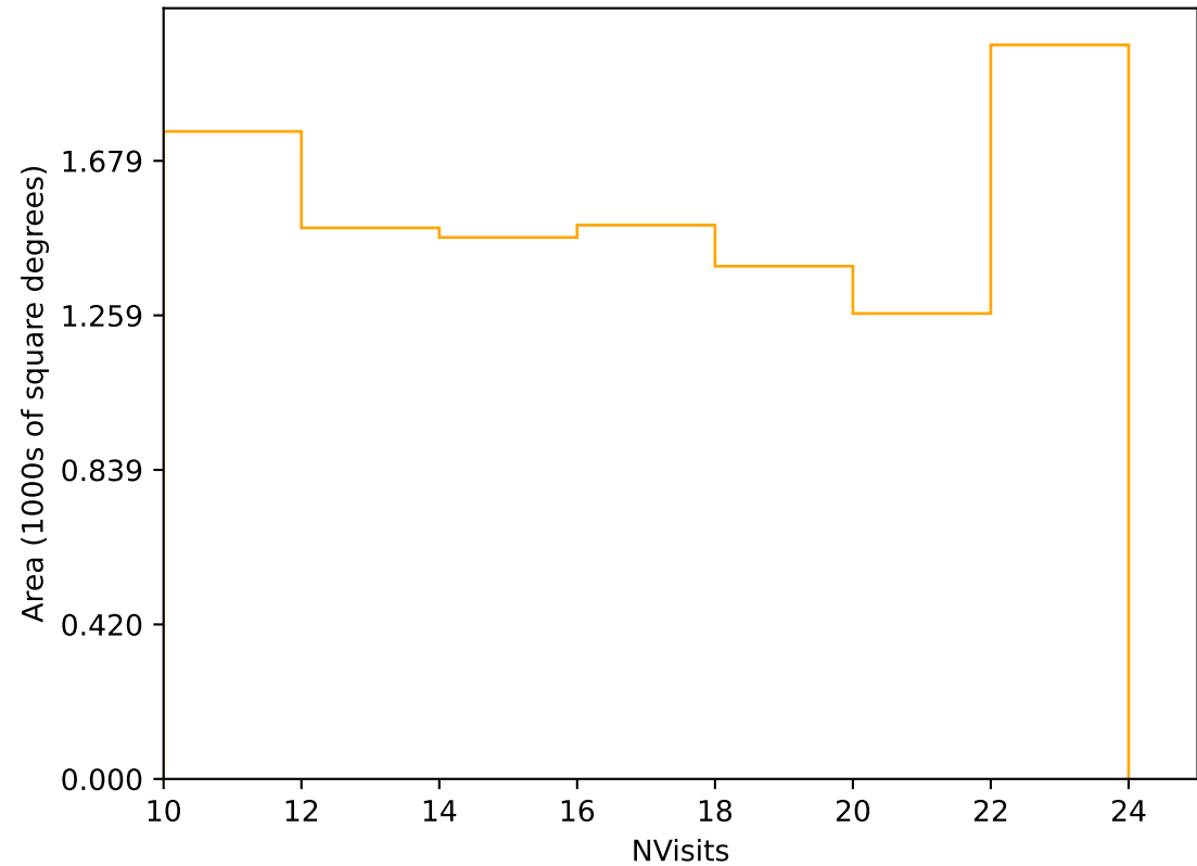
internal_u_expt38_nscale1.1v3.4_10yrs Yr 3-4 r band: NVisits
