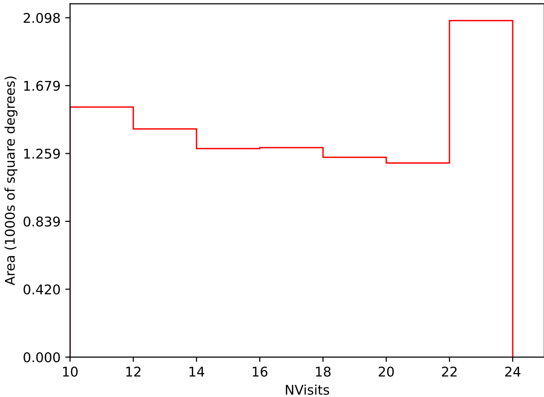
internal_u_expt38_nscale1.1v3.4_10yrs Yr 3-4 i band: NVisits
