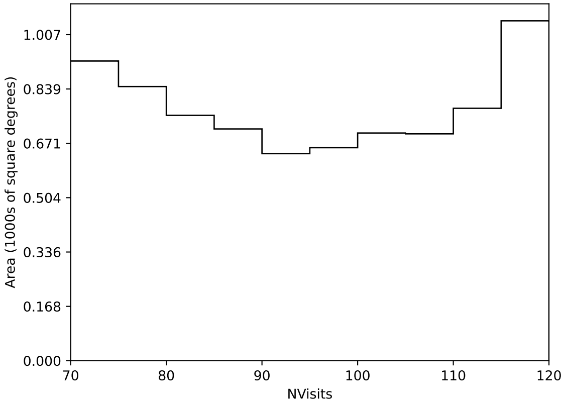
internal_u_expt38_nscale1.1v3.4_10yrs Yr 3-4 all bands: NVisits
