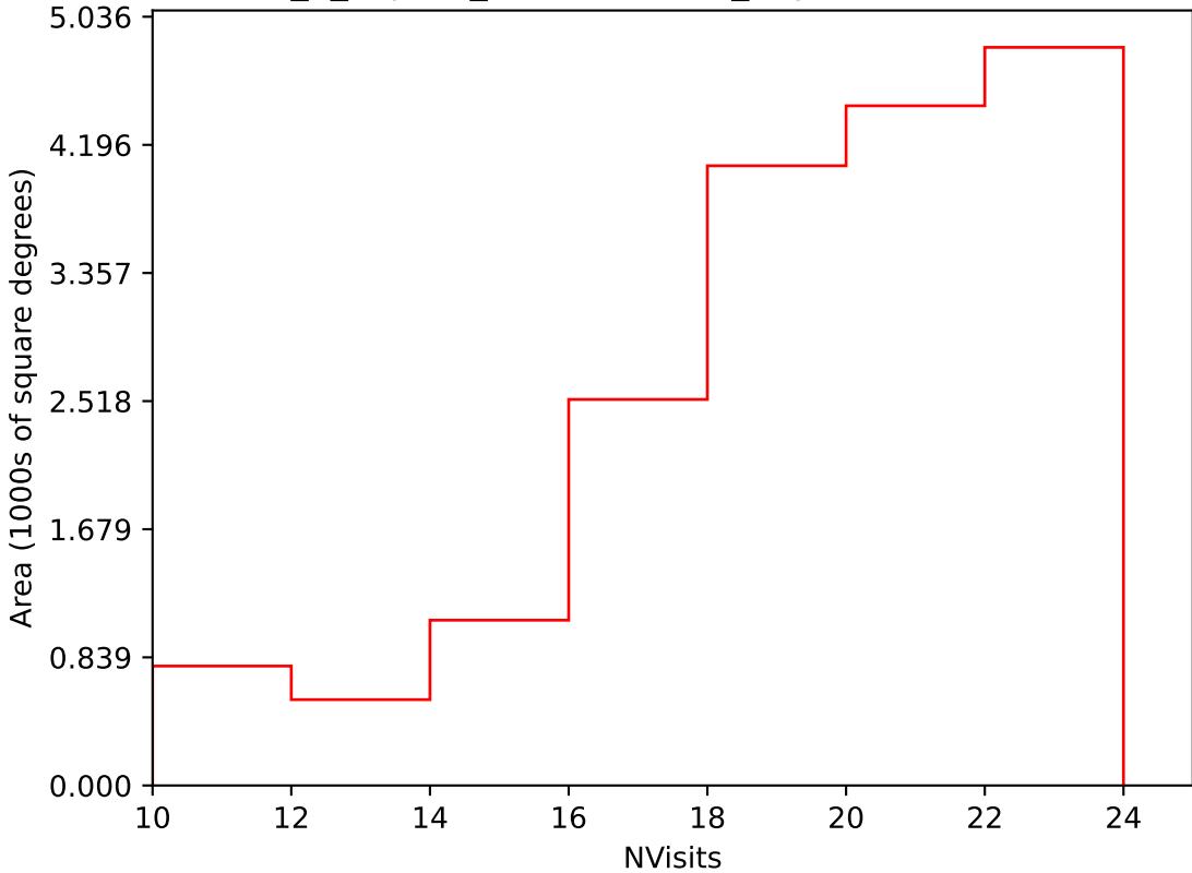
internal_u_expt38_nscale1.1v3.4_10yrs Yr 1 i band: NVisits
