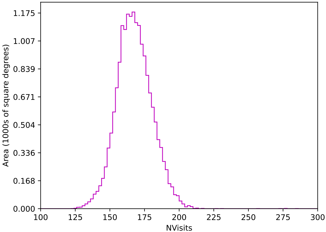
internal_u_expt38_nscale1.1v3.4_10yrs WFD z band: NVisits
