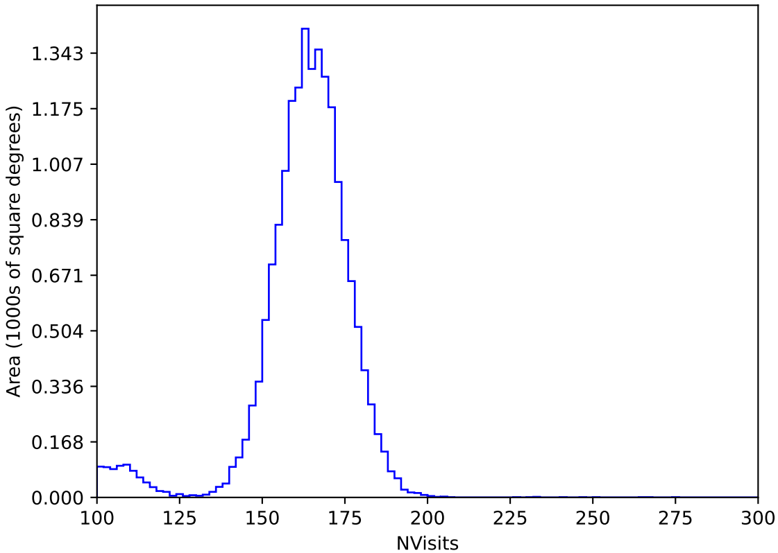
internal_u_expt38_nscale1.1v3.4_10yrs WFD y band: NVisits
