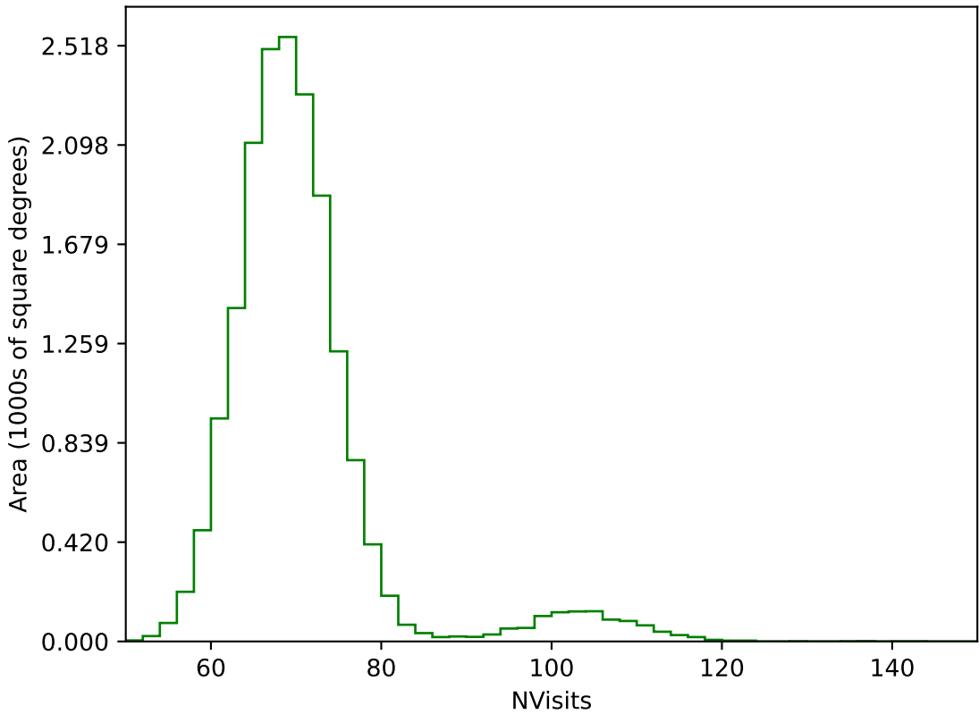
internal_u_expt38_nscale1.1v3.4_10yrs WFD g band: NVisits
