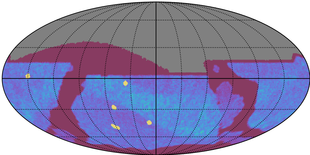
internal_u_expt38_nscale1.1v3.4_10yrs All sky z band: NVisits
