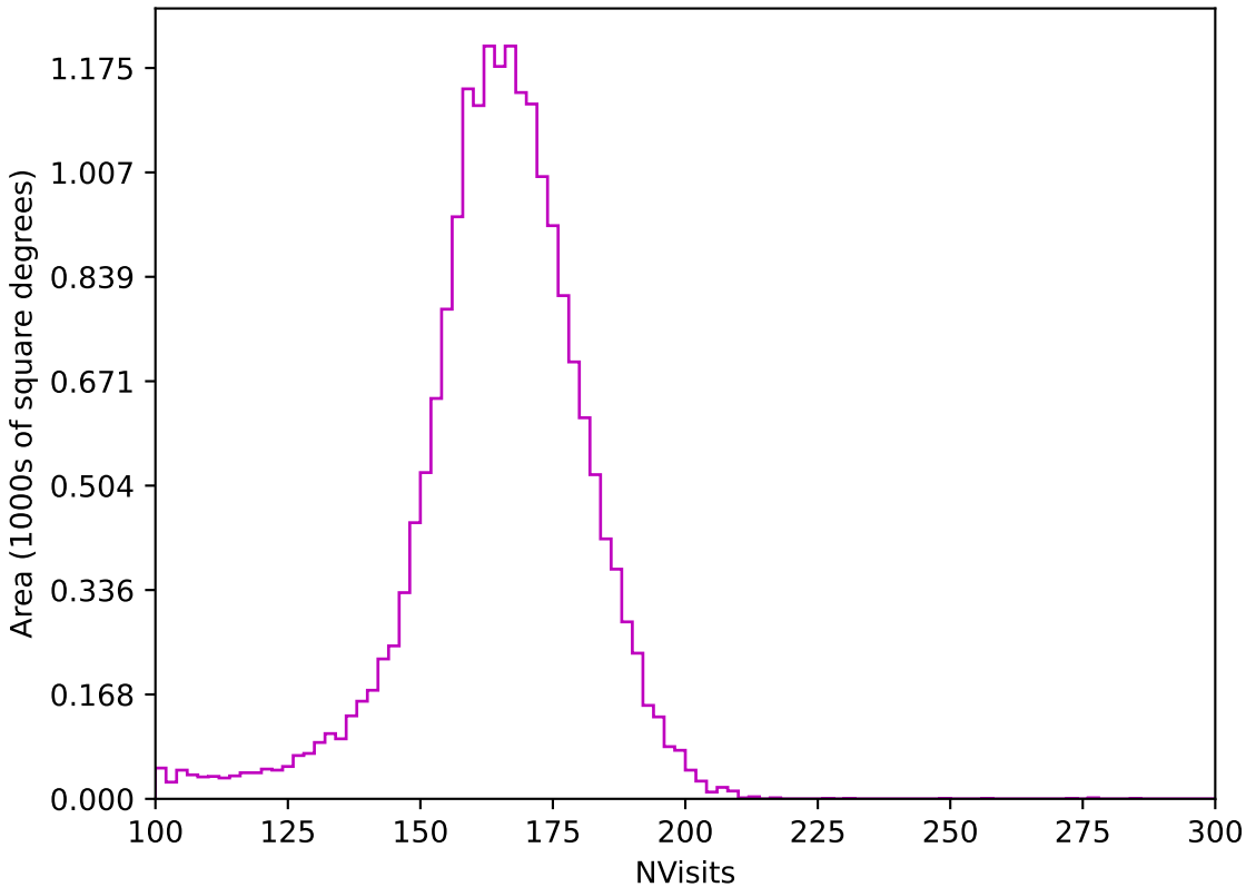
internal_u_expt38_nscale1.1v3.4_10yrs All sky z band: NVisits
