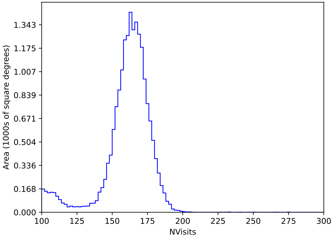
internal_u_expt38_nscale1.1v3.4_10yrs All sky y band: NVisits
