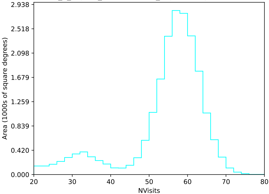
internal_u_expt38_nscale1.1v3.4_10yrs All sky u band: NVisits
