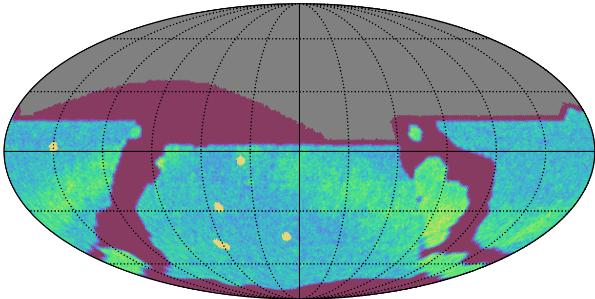
internal_u_expt38_nscale1.1v3.4_10yrs All sky r band: NVisits
