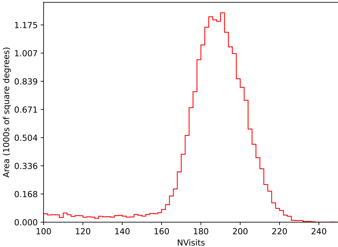
internal_u_expt38_nscale1.1v3.4_10yrs All sky i band: NVisits
