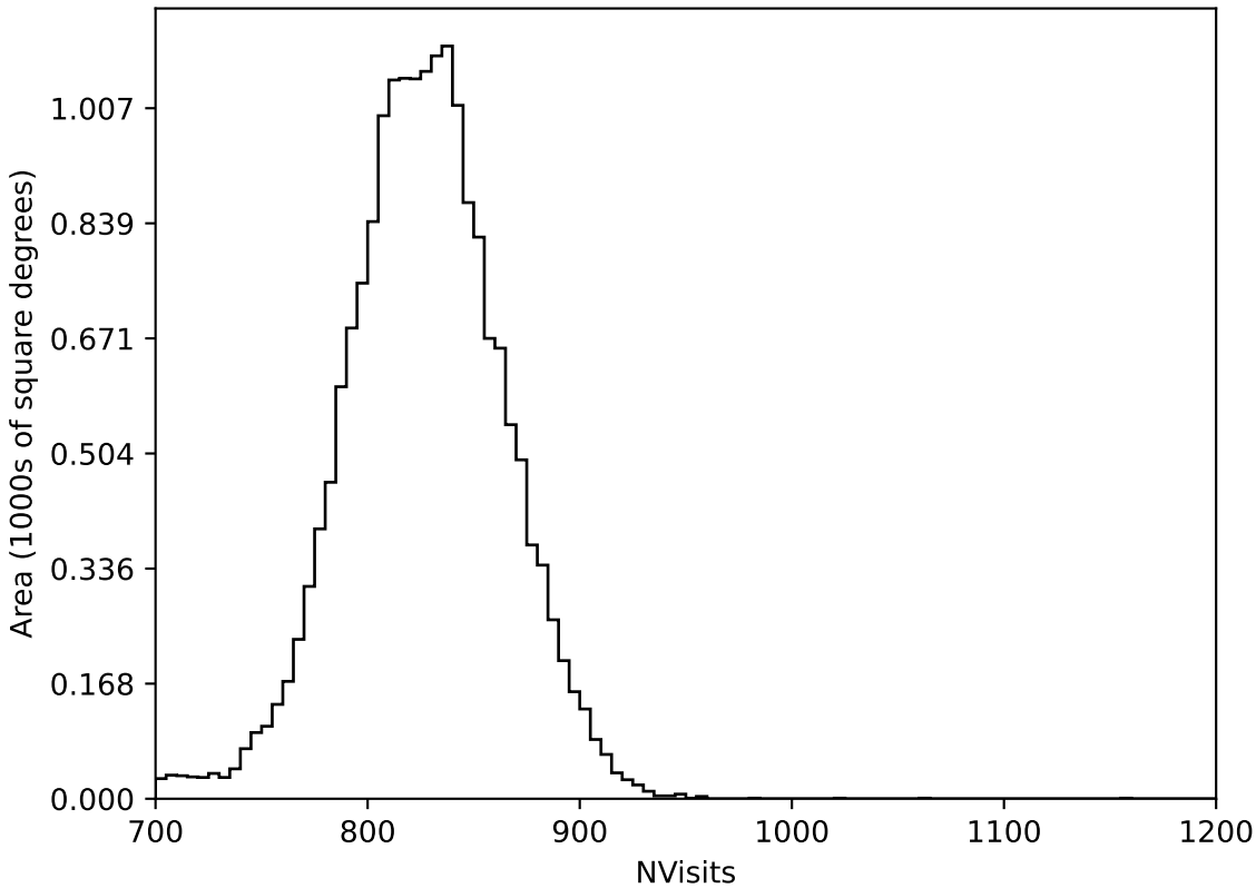
internal_u_expt38_nscale1.1v3.4_10yrs All sky all bands: NVisits
